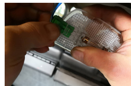
Disconnect the plug connection while actuating the latch on the plug.
